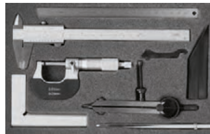
analog
