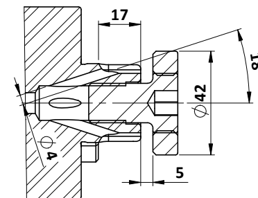
SECTION F-F (1:1.5)
