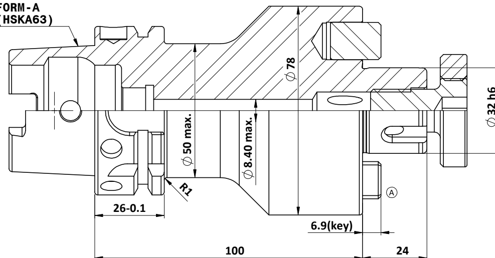
SECTION F-F (1:1.5)
