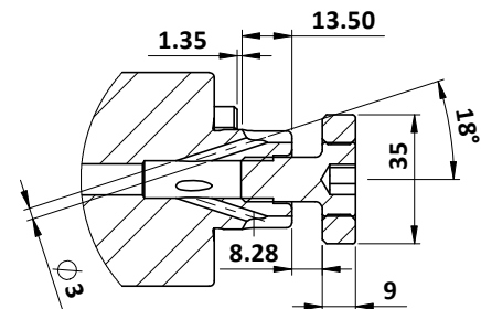
SECTION A-A (1:1.6)
