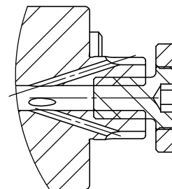
SECTION B-B SCALE 1 : 1.8
