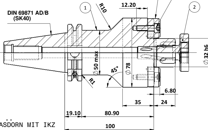
SECTION A-A (1:1.8)
