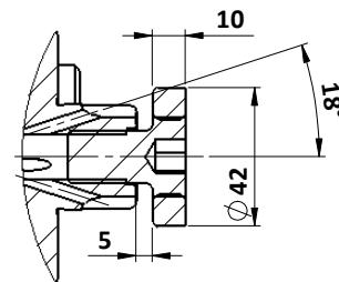
SECTION A-A (1:1.8)
