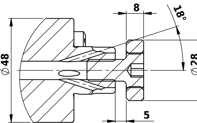
SECTION E-E (1 : 1.2)
